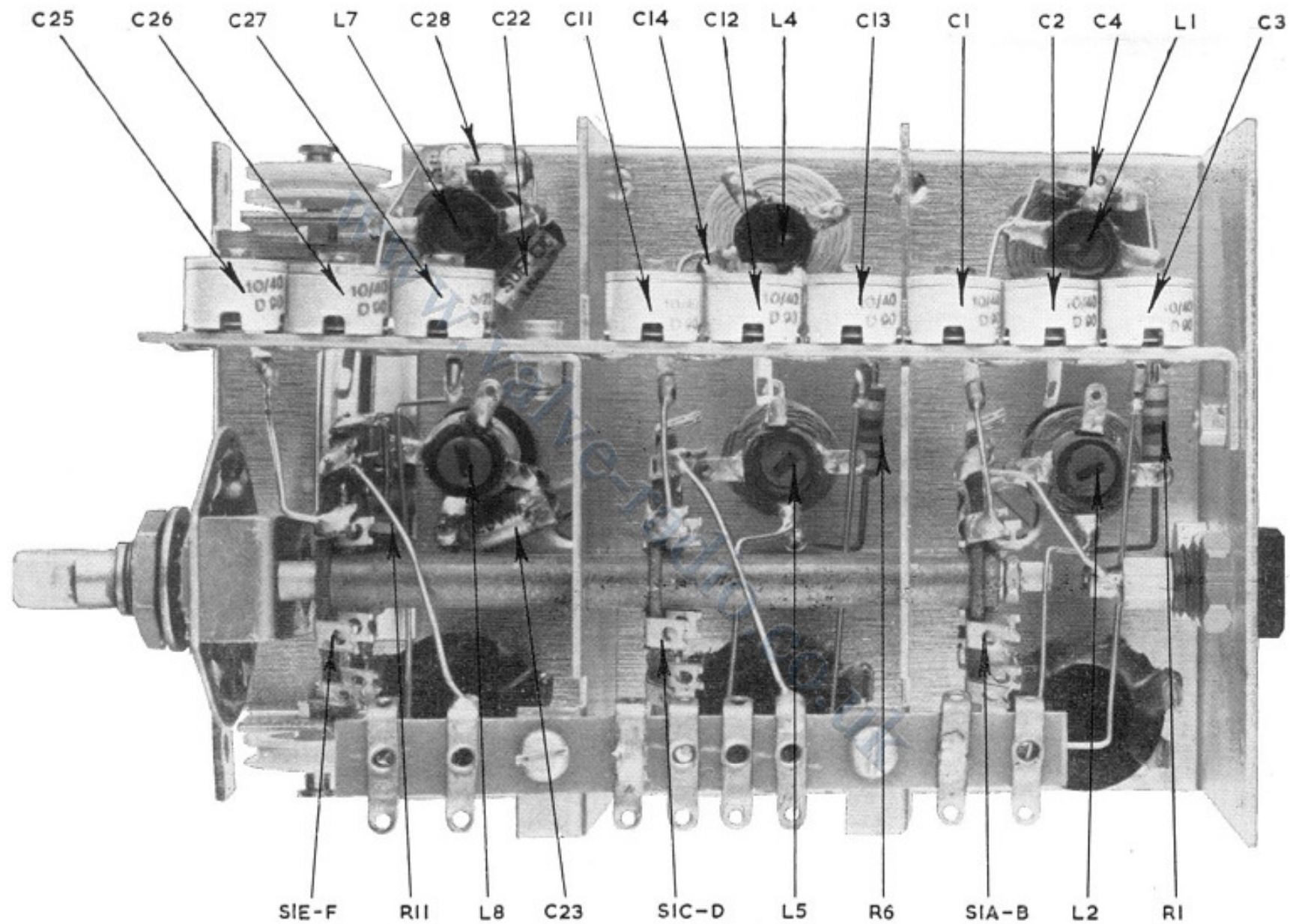
LAYOUT PHOTOGRAPH B — RF CHASSIS (EUROPEAN)
