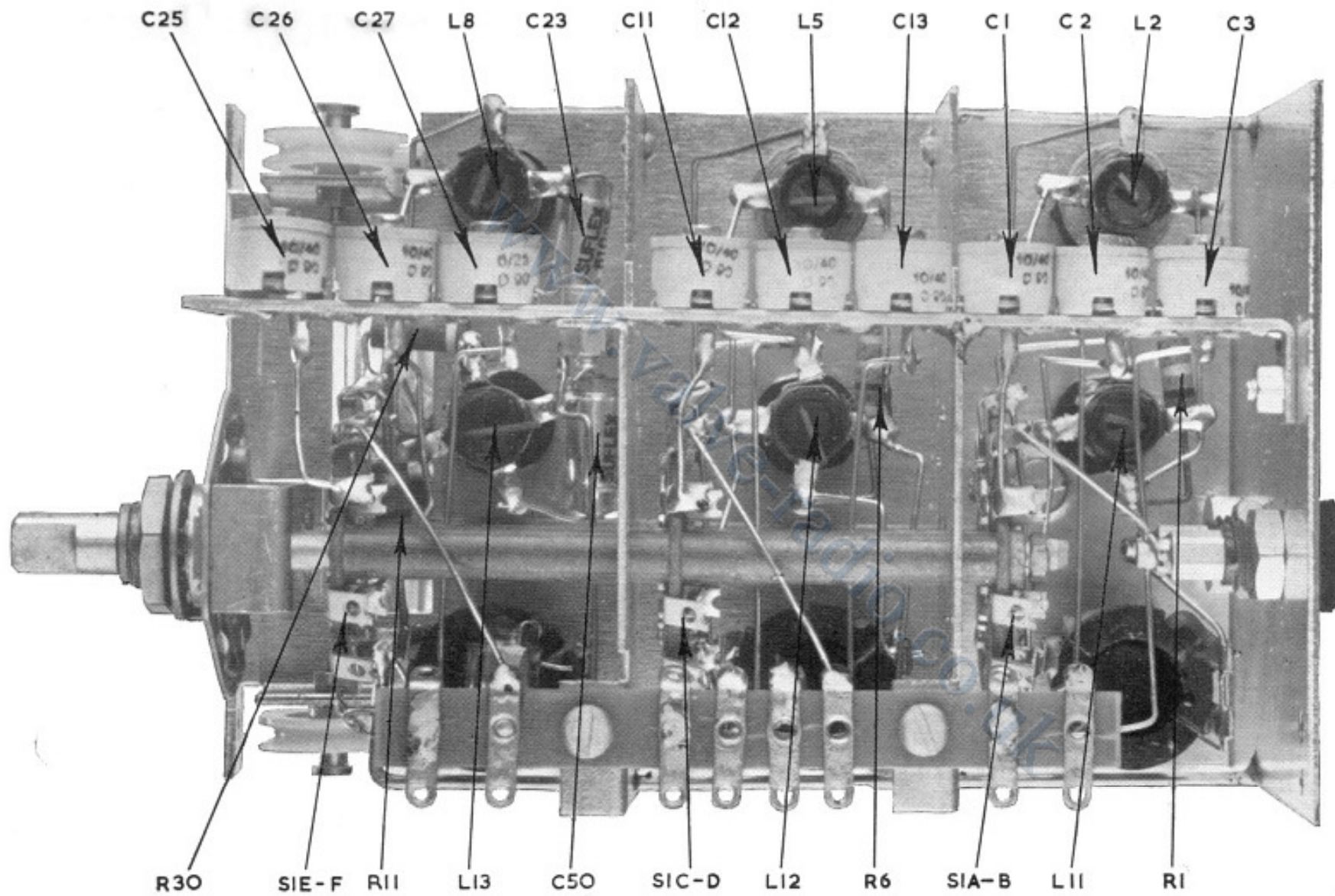
LAYOUT PHOTOGRAPH C — RF CHASSIS (OVERSEAS)
