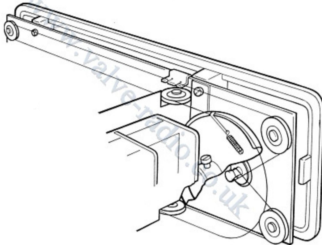
DRIVE CORD ASSEMBLY
