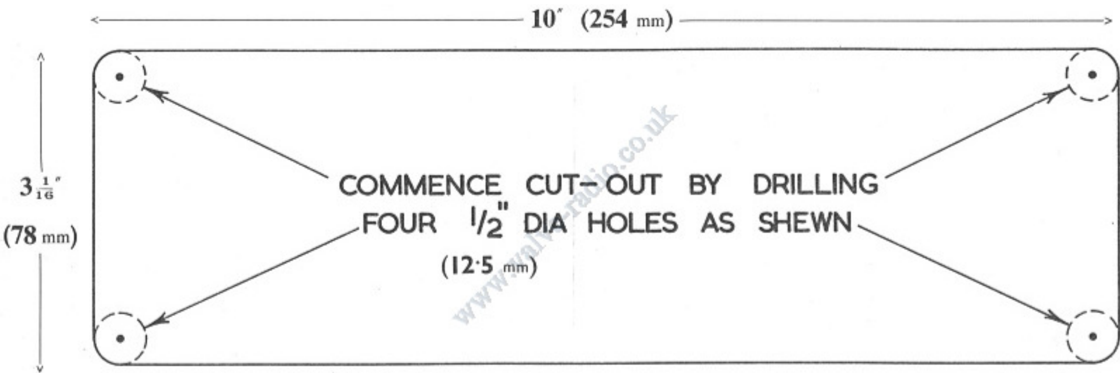
CUT-OUT TEMPLATE FOR QUAD CONTROL UNITS & TUNERS
