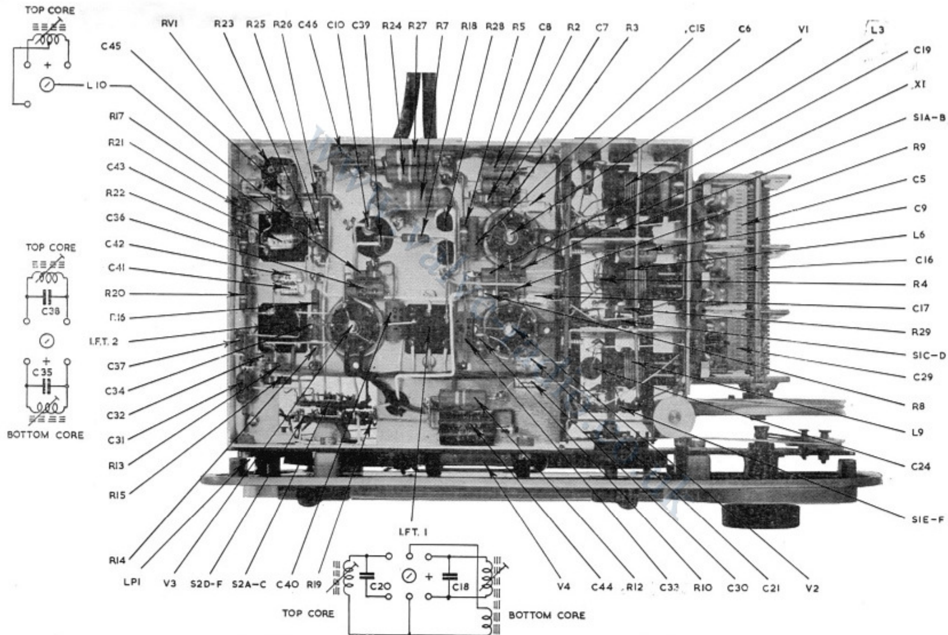
LAYOUT PHOTOGRAPH A — CHASSIS UNDERSIDE
