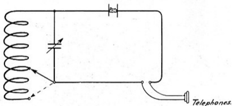
Diagrammatic View of Wavemeter.
