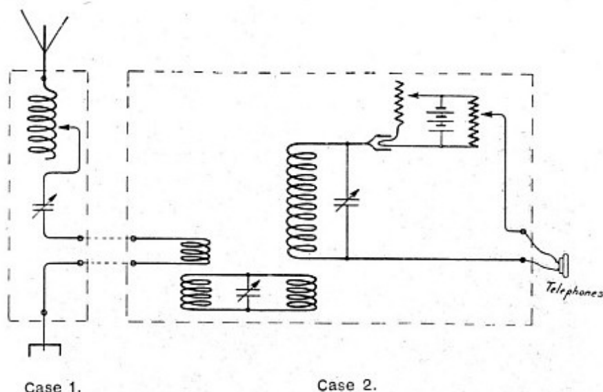
Diagrammatic View of Connections for Valves.
