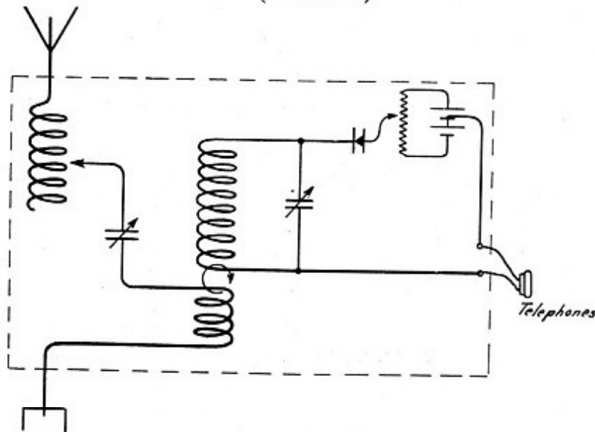
Diagrammatic View of Connections of Crystal Receiver.
