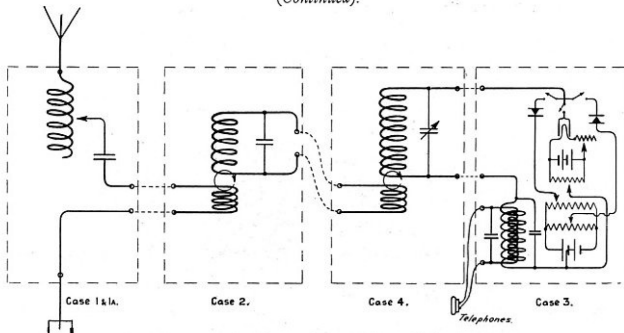
Diagrammatic View of Connection of Receiver.
