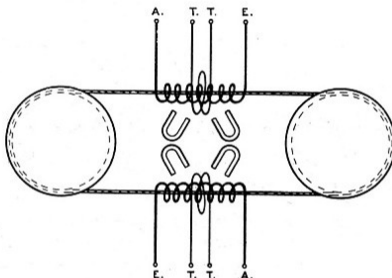
Diagrammatic View of Marconi's Magnetic Detector.
