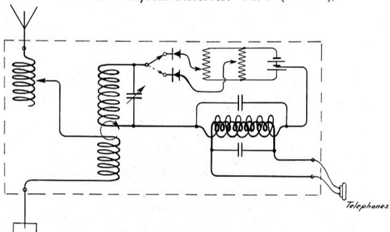
Diagrammatic View of Crystal Receiver Connections.
