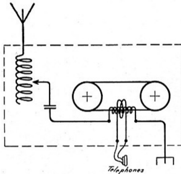
Diagrammatic View of Connections of Receiver.
