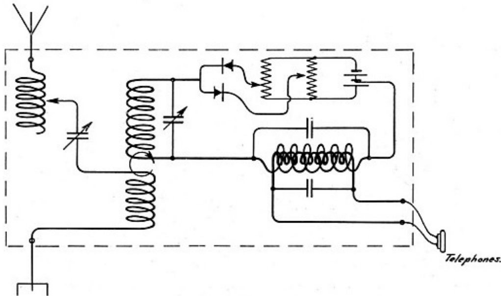
Diagrammatic View of Connection in Receiver.
