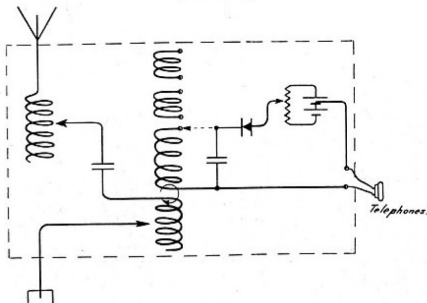
Diagrammatic View of Connections of Receiver.
