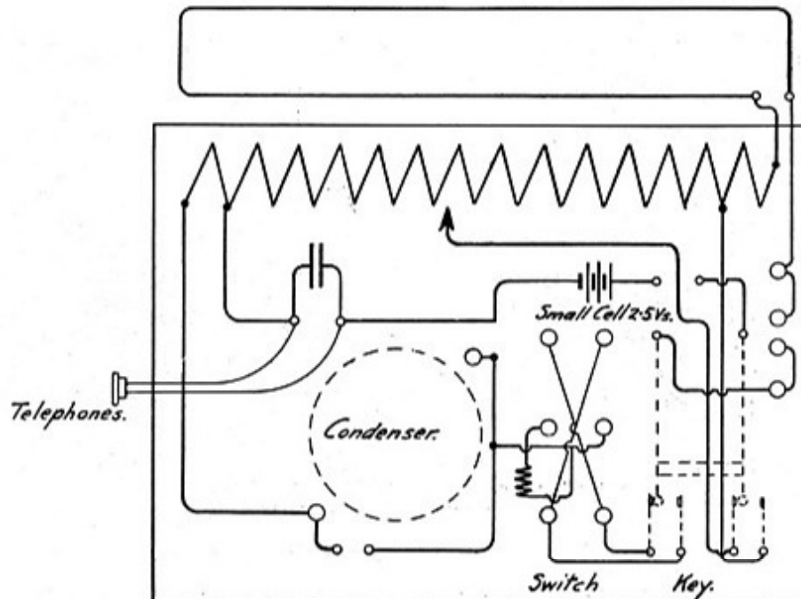
Diagrammatic View of Connections of Decremeter.
