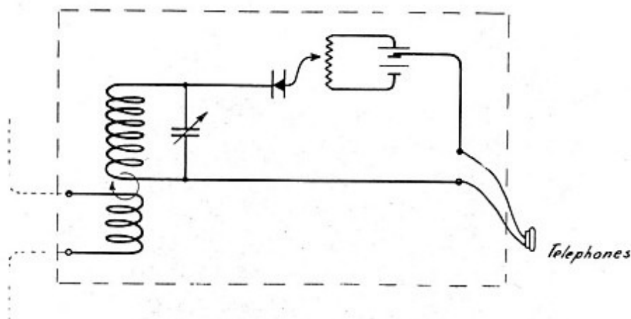
Diagrammatic View of Crystal Receiver Connections.
