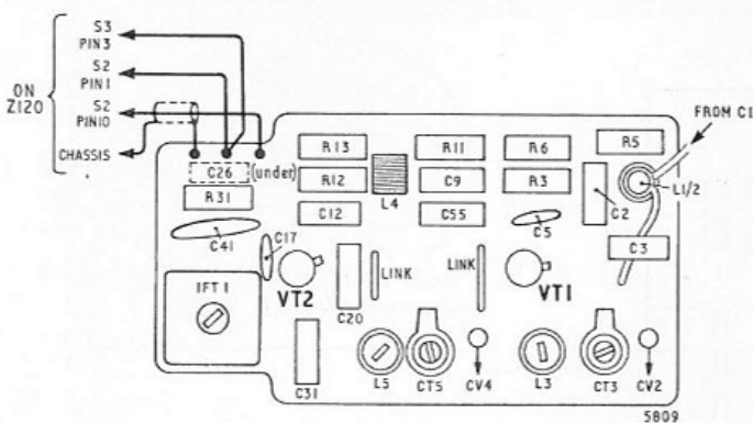
Fig. 4a V.H.F. unit (A778) component layout
