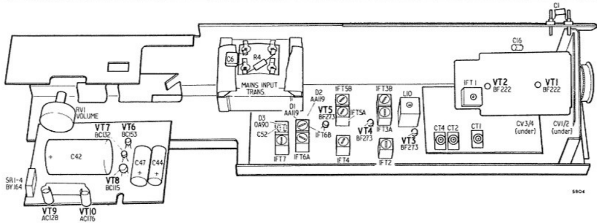
Fig. 1 Rear view of chassis
