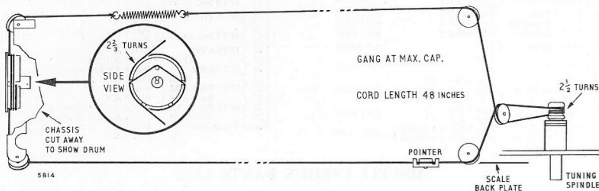
Fig. 8 Cord drive
