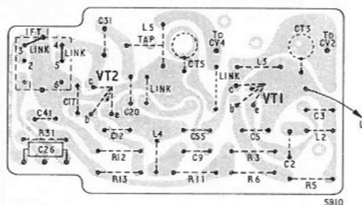
Fig. 4b V.H.F. unit (A778) printed side
